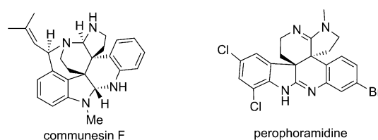
Figure 1. Naturally occurring polycyclic spiroindolines.
