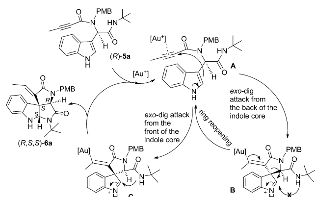
Scheme 2. Proposed mechanism for the diastereoselective domino cyclization to spiroindolines. PMB = p -methoxybenzyl.
